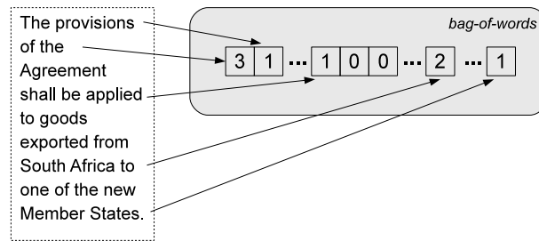
Fig. 1. Bag-of-words representation
